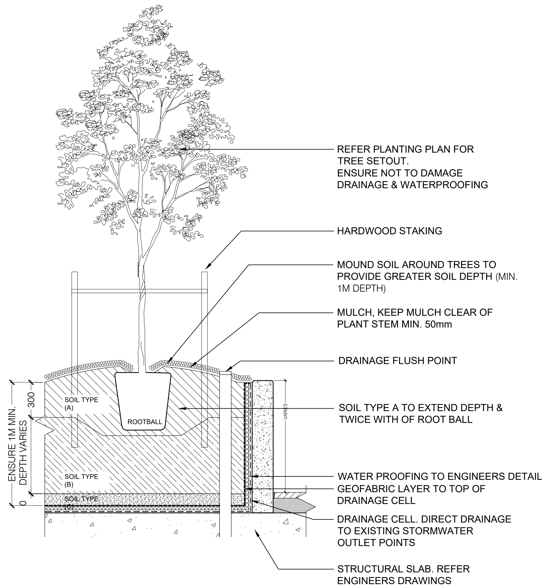
02 TYPICAL TREE PLANTING ON PODIUM DETAIL
