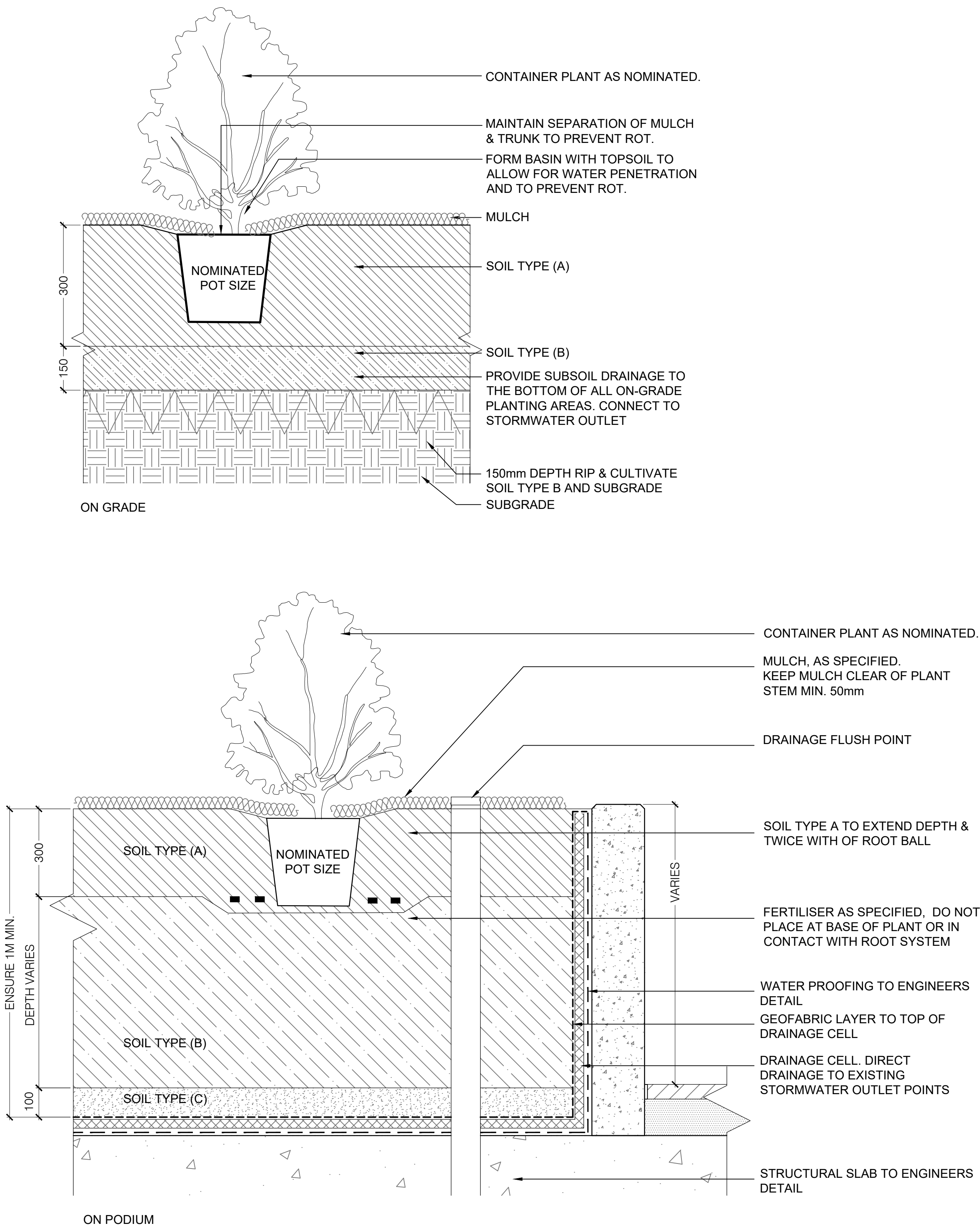
01 TYPICAL SHRUB & GROUND COVER PLANTING DETAILS
