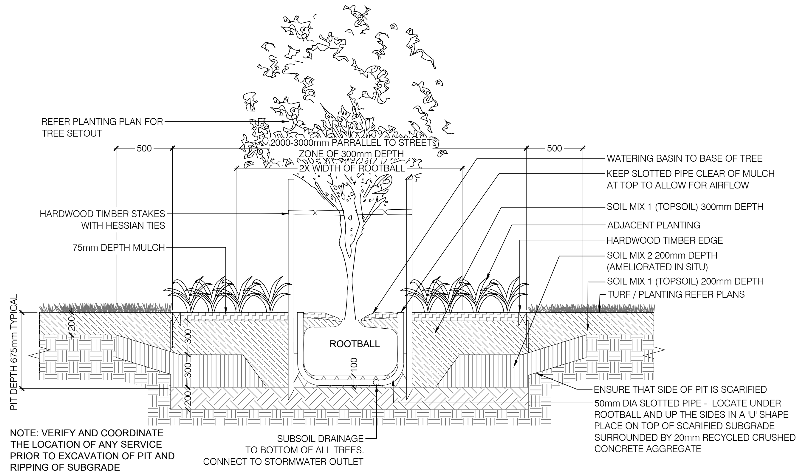
01 TYPICAL STREET TREE PLANTING (NORTH ROAD) - SCALE 1:20 @ A1; 1:40 @ A3
